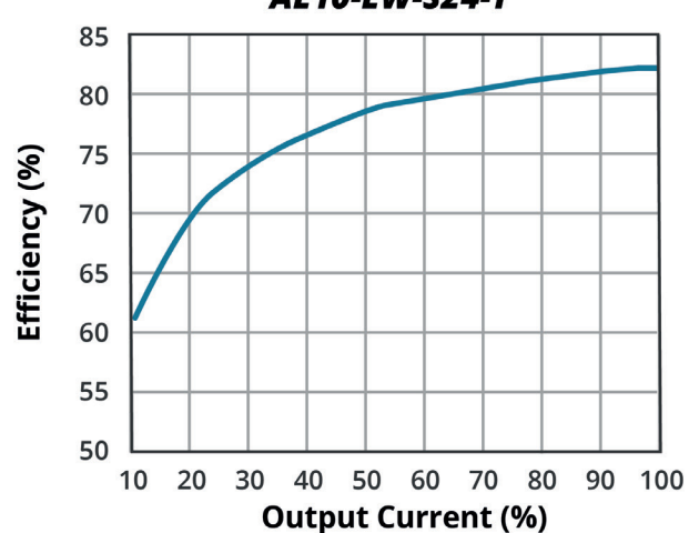
EFFICIENCY VS OUTPUT LOAD AE10-EW-S24-T
